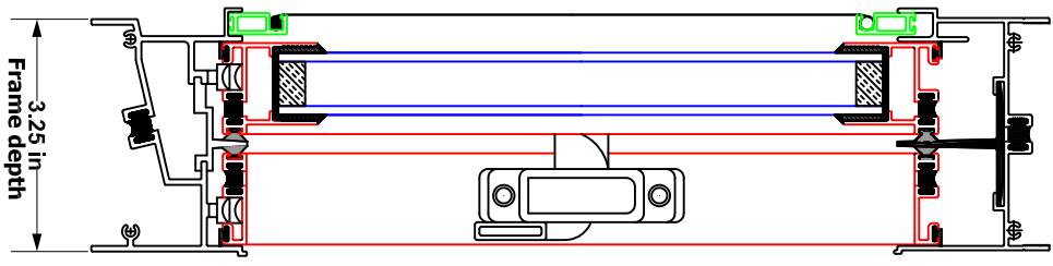
VERTICAL SECTION A-A
